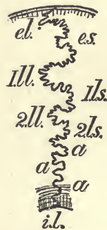
Fig. 107.—Suture-line of an Ammonite ( Harporceras ). The mouth lies to the right. e.l. , External lobe, bisected by a median saddle on the keel. e.s. , External saddle. 1.l. , 1st lateral lobe. 1.s. , 1st lateral saddle. 2.l. , 2nd lateral lobe. 2.s. , 2nd lateral saddle. a , Auxiliary lobes and saddles. i.l. , unseen Internal lobe.
